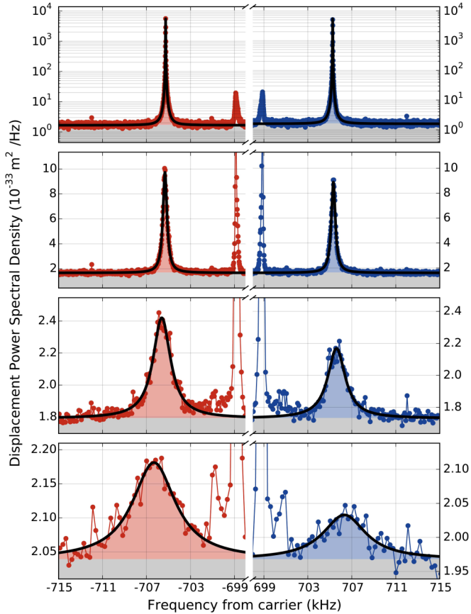
FIG. 2. (Color online) Motional sidebands of the mechanical oscillator. The membrane's displacement power spectral density S_{xx} is plotted versus the measurement frequency \omega . The red data (left panels) show the red sideband S_{xx}^{(r)} , and the blue data (right panels) show the blue sideband S_{xx}^{(b)} . From top to bottom, the cooling laser power is P_{CL} = 0, 34, 158, 415 \mu\text{W} . The black line is the fit described in the text. The red/blue shading indicates the Lorentzian portion of the fit, specified by \tilde{\omega} , \tilde{\gamma} , s^{(r)} , and s^{(b)} . The gray shading indicates the fitted noise floor (shot noise plus dark noise), specified by b^{(r)} and b^{(b)} . The detuning of the probe beam causes the displacement imprecision to differ slightly between the red and blue data; as a visual guide, the vertical axes are shifted to compensate for this difference. The data was fit over the range 702 \text{ kHz} \leq |\omega/2\pi| \leq 714 \text{ kHz} . As P_{CL} increases, laser cooling causes the sidebands to broaden and shrink. In the lowest panel, the ratio of their areas is \xi + 1 = 2.18 \pm 0.32 , corresponding to \bar{n} = 0.84 \pm 0.22 .
