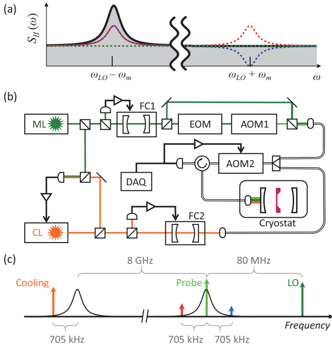
FIG. 1. (Color online) Schematic of the measurements. (a) Contributions to the heterodyne measurement described in the text. Contributions from the shot noise (green), the oscillator's zero-point motion (red), and the oscillator's response to the quantum fluctuations of the cavity field (blue) are shown in the vicinity of the red sideband (left) and the blue sideband (right). The total signal is the black curve. (b) The experimental setup. Free-space beams, optical fibers, and electrical circuits are colored lines, hollow lines, and thick black lines, respectively. Beams from two lasers (ML, CL) pass through filter cavities (FC1, FC2). The probe beam is shifted by AOM1, while AOM2 tracks fluctuations in the cryogenic cavity. Light is delivered to (and collected from) the cryostat by a circulator. Control circuits, photodiodes, and fiber couplers are indicated by triangles, semicircles, and ovals, respectively. The mechanical oscillator is shown in purple. (c) The spectrum of the lasers (orange, light green, and dark green), cavity modes (black), and mechanical sidebands (red and blue).
