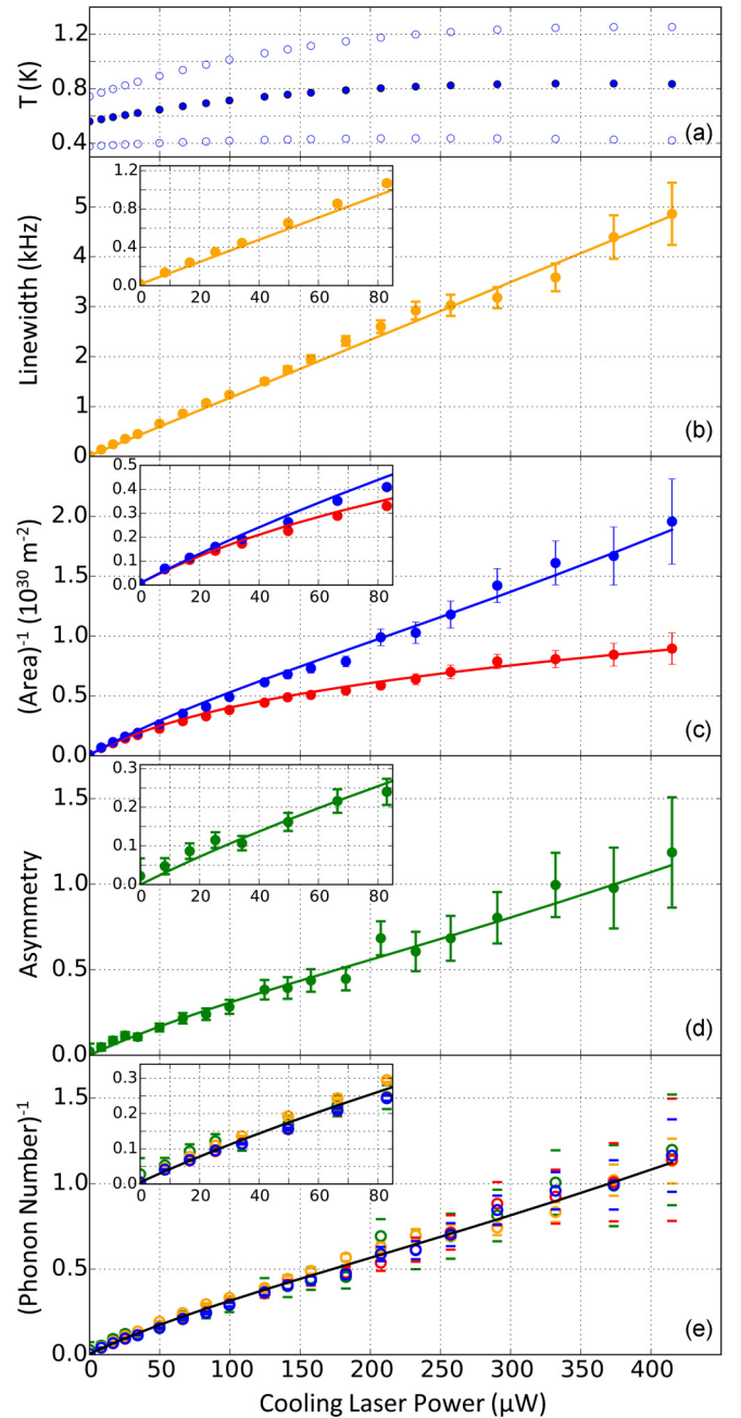
FIG. 3. (Color online) Behavior as a function of cooling laser power P_{CL} . (a) Temperature recorded by two thermometers ( T_{\text{pot}} and T_{\text{stage}} , hollow points) and the membrane's inferred bath temperature T_{\text{bath}} (solid points). Note T_{\text{pot}} < T_{\text{stage}} . (b) Mechanical linewidth \tilde{\gamma}/2\pi . (c) Inverse area of each sideband, 1/A^{(r)} and 1/A^{(b)} . (d) Sideband asymmetry \xi . (e) Inverse mean phonon number 1/\bar{n} , determined from \xi (green), A^{(r)} (red), A^{(b)} (blue), and \tilde{\gamma} (yellow). Solid lines in (b)–(e) are calculated values, as described in the text. Each inset shows a detailed view of the data for low P_{CL} .
