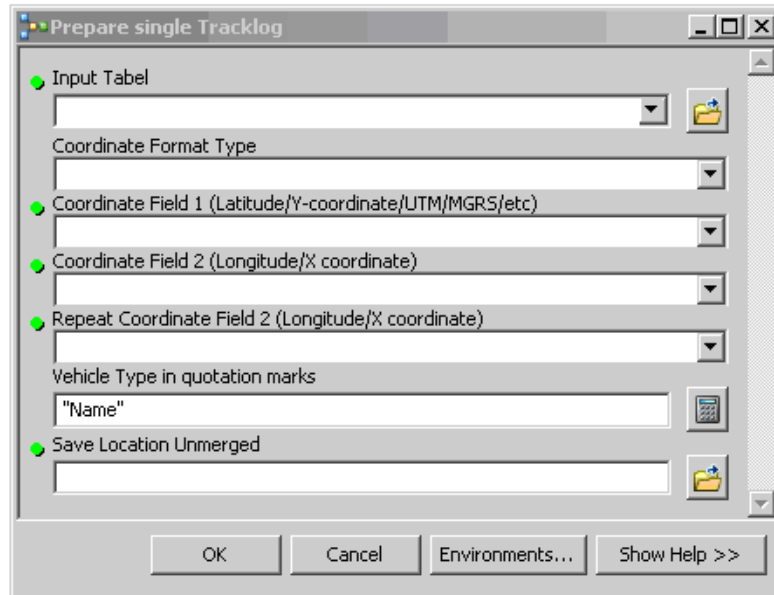
FIGUR 30: DEL 1- DIALOGBOKS
