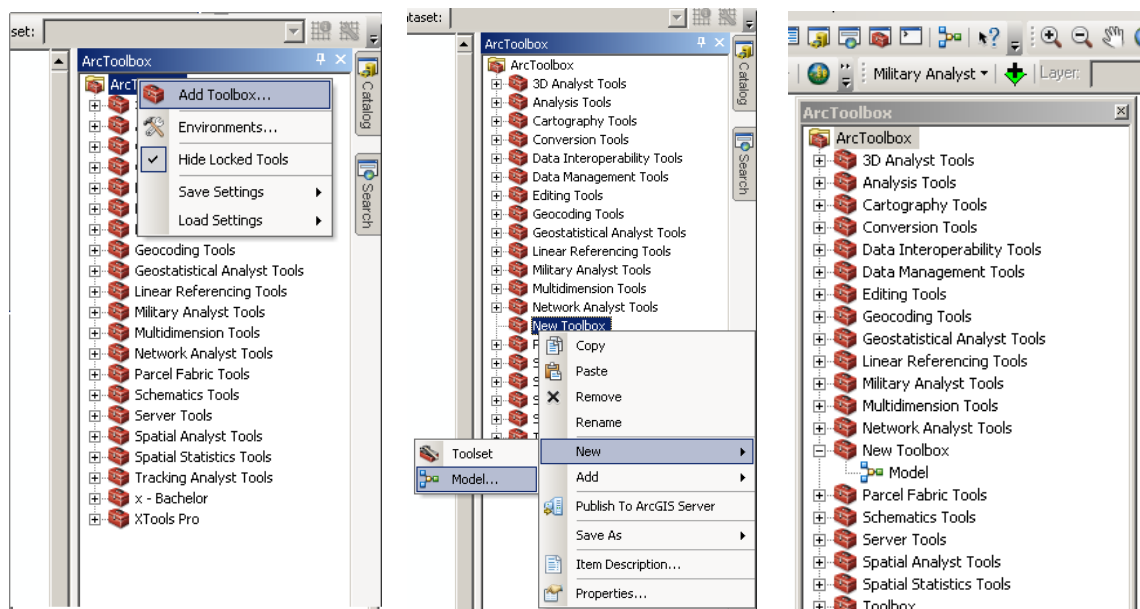
FIGUR 1: ARCTOOLBOX
