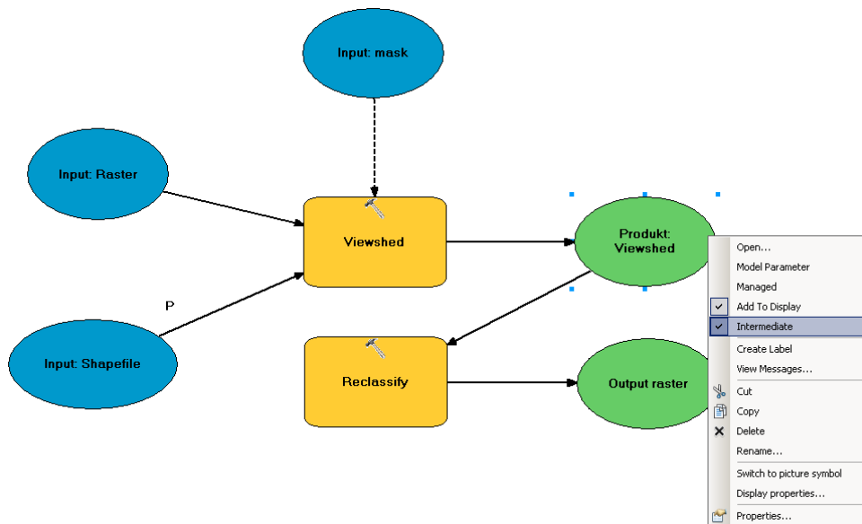
FIGUR 7: MODELBUILDER - HURTIGMENY
